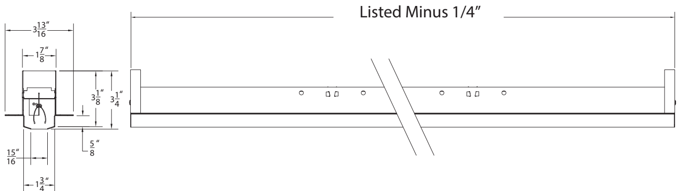
SECTION B-B SCALE 1/3
